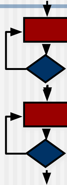
Concatenated Loops
