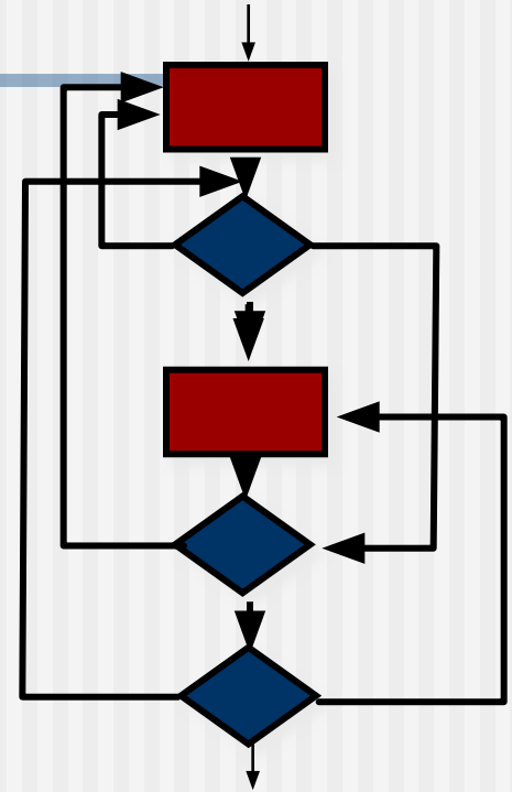
Unstructured Loops
