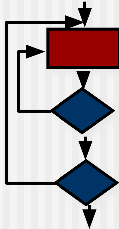
Nested Loops
